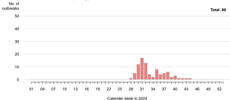
Outbreaks per calender week: GREECE Reporting period: 2024-01-01 – 2024-12-31, as of: 2025-01-20
