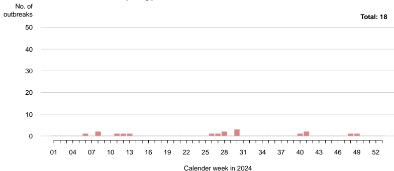
Outbreaks per calendar week: TURKEY Reporting period: 2024-01-01 – 2024-12-31, as of: 2025-01-20
